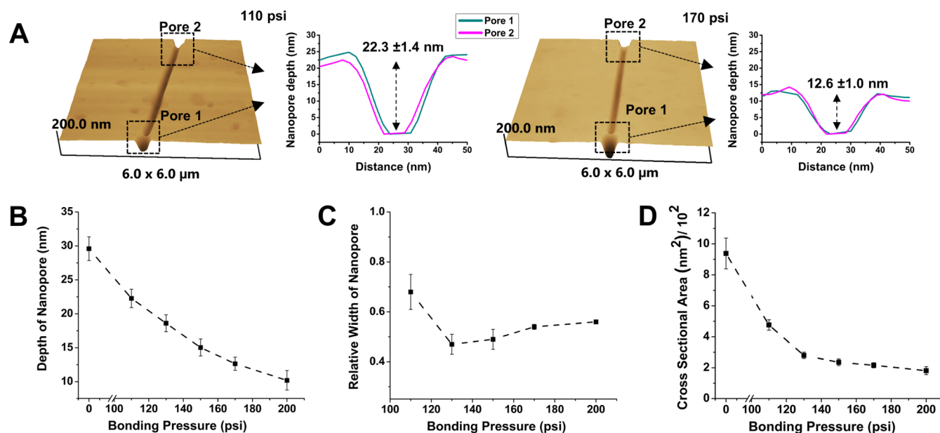
Figure 2. Nanopore depth and width with varying thermal fusion bonding pressure. (A) AFM scans of PMMA devices at 110 and 170 psi bonding pressures. (B) Change in the depth of the in-plane nanopores with bonding pressure. (C) Relative width of the in-plane nanopores after bonding at different pressures relative to the width of the nanopore before bonding (0 psi). There was no statistical difference in relative width from 130 to 200 psi at the 95% confidence interval ( p > 0.05 ). (D) Cross-sectional area of the in-plane nanopore with thermal fusion bonding pressure.
