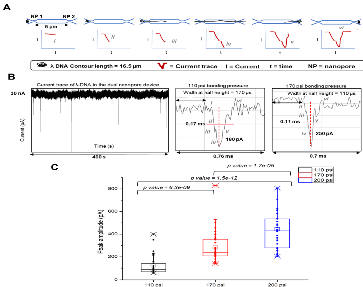
Figure 3. \lambda -DNA translocation through the dual in-plane PMMA nanopores and the ramifications of the size of the nanopore on peak amplitude. (A) Schematic of the \lambda -DNA translocation through the in plane dual nanopore device that gives rise to a negative peak as the DNA enters the first pore. Since the contour length of the DNA is longer than both the pores, there is a second subsequent peak when the DNA coresides in both the pores. The DNA then leaves the pores very quickly which makes the current return to the baseline. (B) Detected current transient trace typically observed in a time interval of 400 s as a result of \lambda -DNA translocation and magnified images of individual peak shapes at various translocation stages of the DNA through the dual nanopore at 110 and 170 psi pressure, respectively. (C) Distribution of peak amplitudes of \lambda -DNA at 110, 170, and 200 psi bonding pressures. The average peak amplitude increases with the increasing bonding pressure. p values calculated between each bonding pressure condition (Wilcoxon signed rank test) show statistically a significant difference at 95% confidence interval ( p < 0.05 ).
