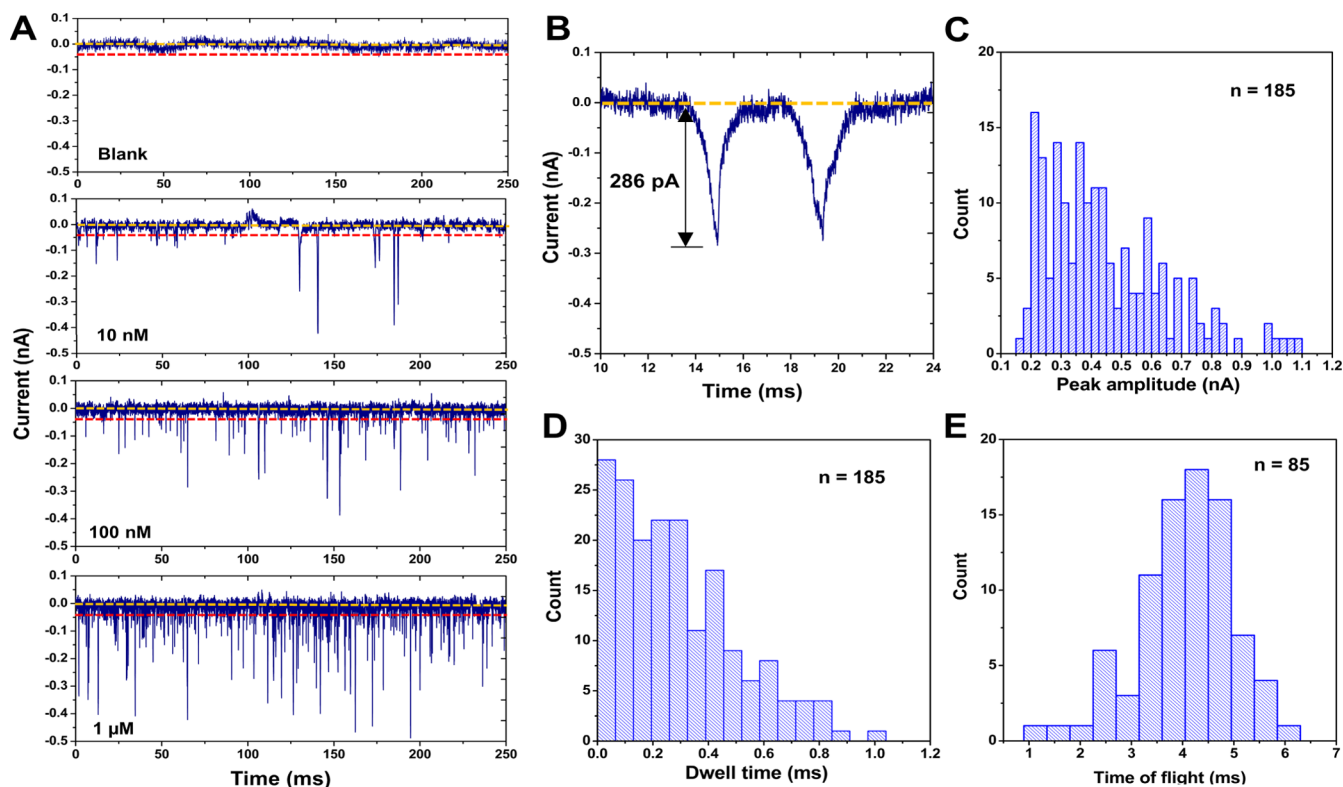
Figure 5. Translocation of rAMPs through dual in-plane nanopore devices assembled at 200 psi bonding pressure. (A) 250 ms current transient trace of signal amplitudes obtained for blank, 10, 100 nM, and 1 \mu M solutions of rAMP using dual in-plane nanopore devices. An increase in event frequency was observed with increasing concentration ( R^2 = 0.9757 ). (B) Example peak pair selected using the peak pair criteria. (C) Peak amplitude distribution of rAMP events. (D) Dwell time distribution for rAMP events. (E) TOF distribution for rAMP.
