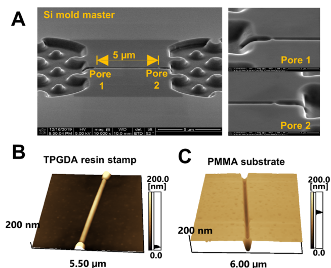
Figure 1. Dual in-plane nanopore device. (A) SEM image of the Si mold master. The two in-plane nanopores are 5 \mu m apart from each other. AFM scans of the (B) TPGDA resin stamp and (C) imprinted PMMA substrate. Tapping-mode AFM scans were acquired at 0.5 Hz scanning frequency using a high aspect ratio tip with a radius of <2 nm.
